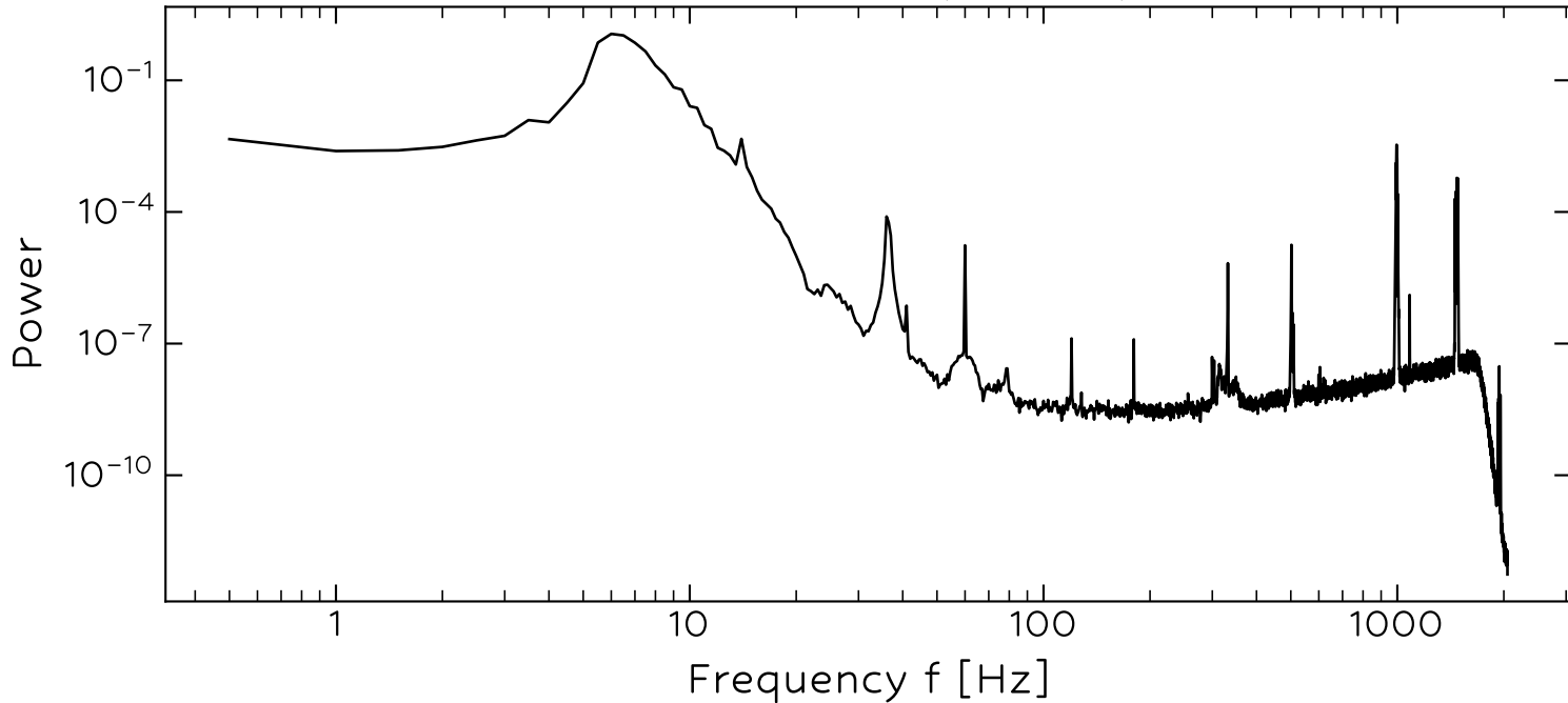
Welch-averaged noise power spectrum
